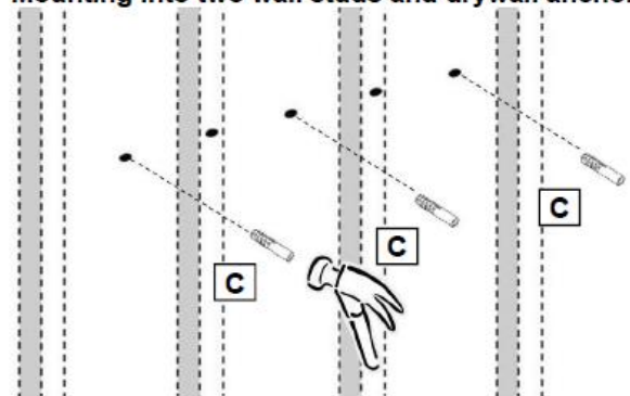
Mounting into two wall studs and drywall anchors
