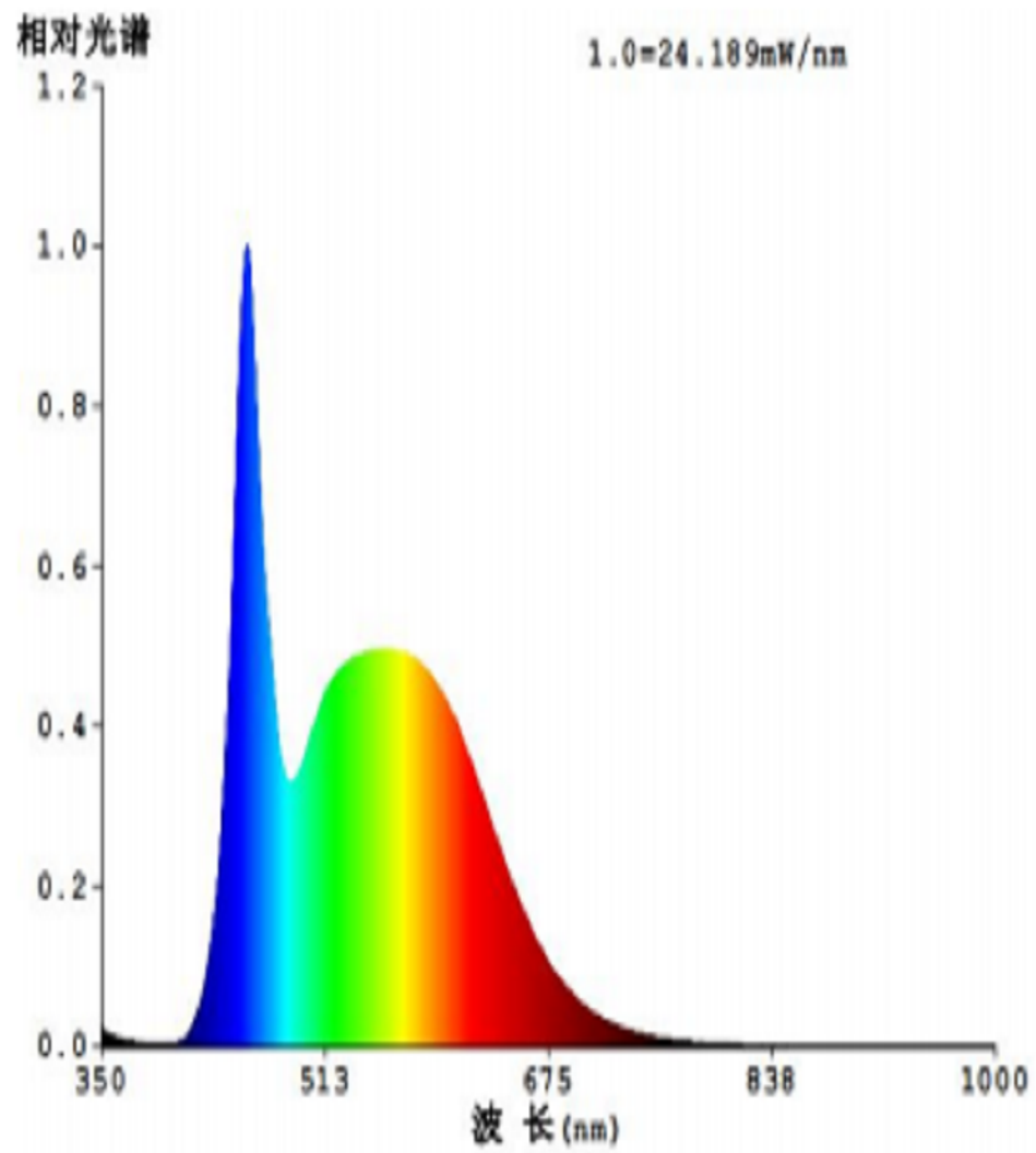
The Spectrum of 6500K
