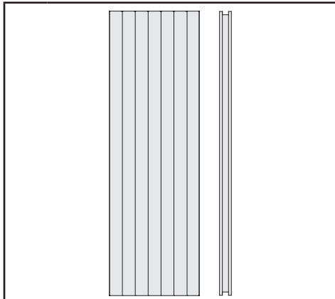
1 x W1 | 1920 x 606 x 68 mm | ID 25548
