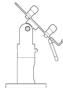
Terminal Stand(x1)
