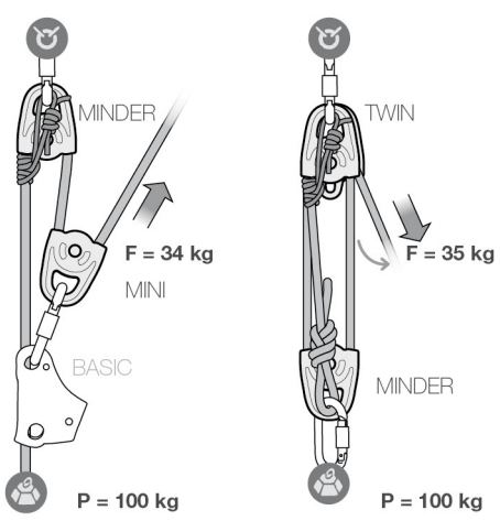
6C. 3:1 hauling system
