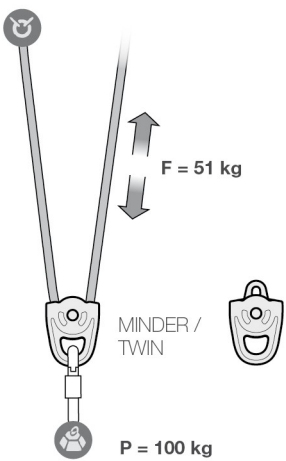
6B. 2:1 hauling system
