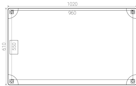
PR0029487-04 (600 Watt)
