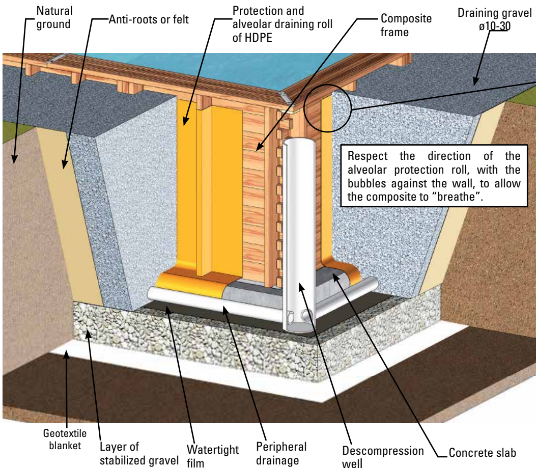
1- Composite frame 2- Roll of alveolar protection a drainage of HDPE
