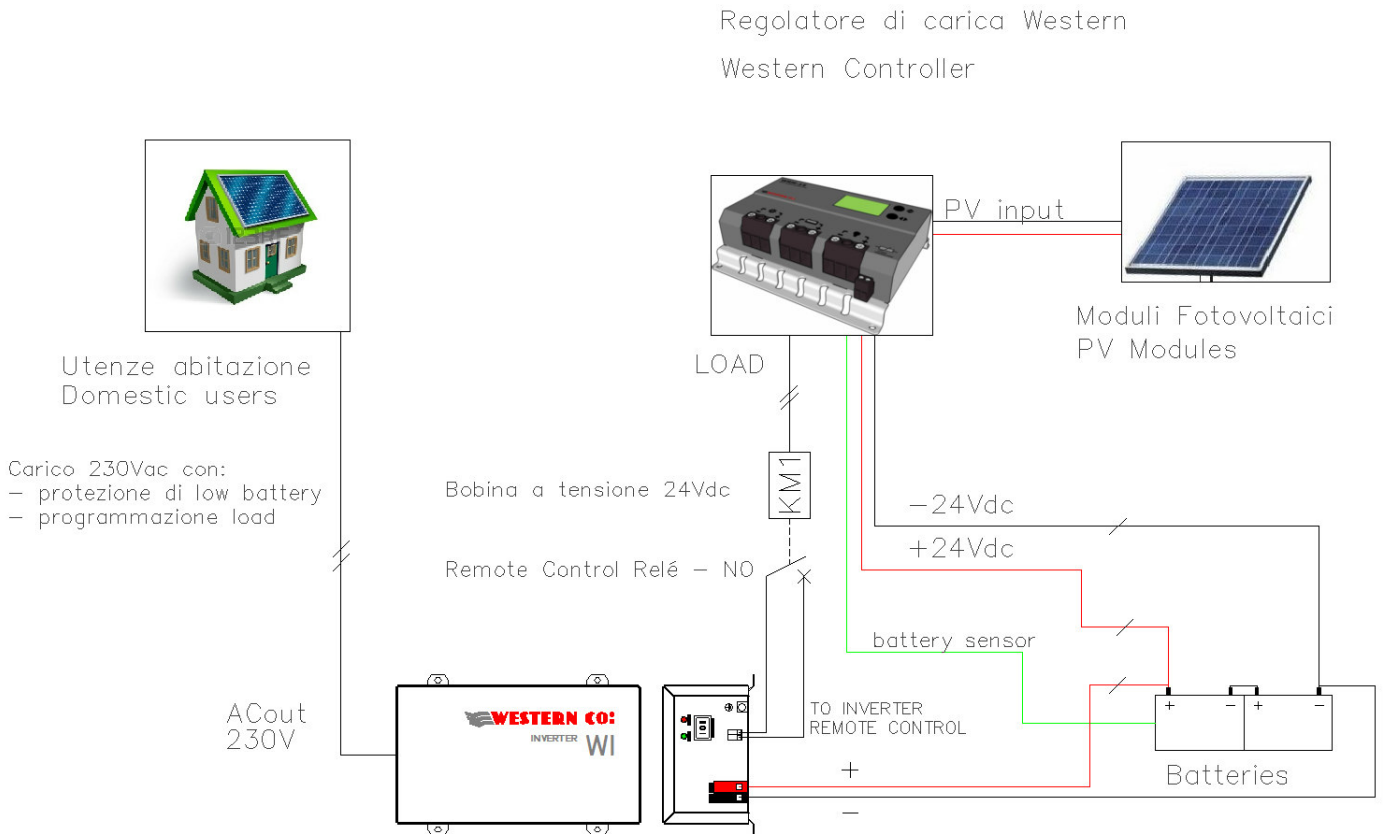
Pic. 4 WI800-24 Wiring scheme
