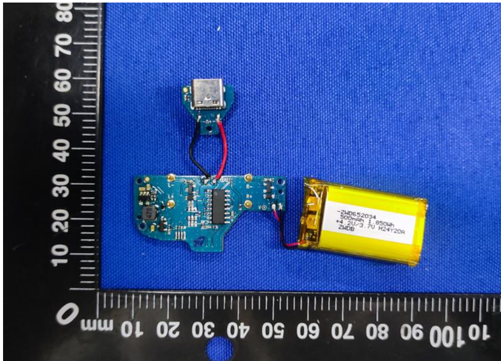
Picture 5 Inside view of battery 图5: 电池内部
