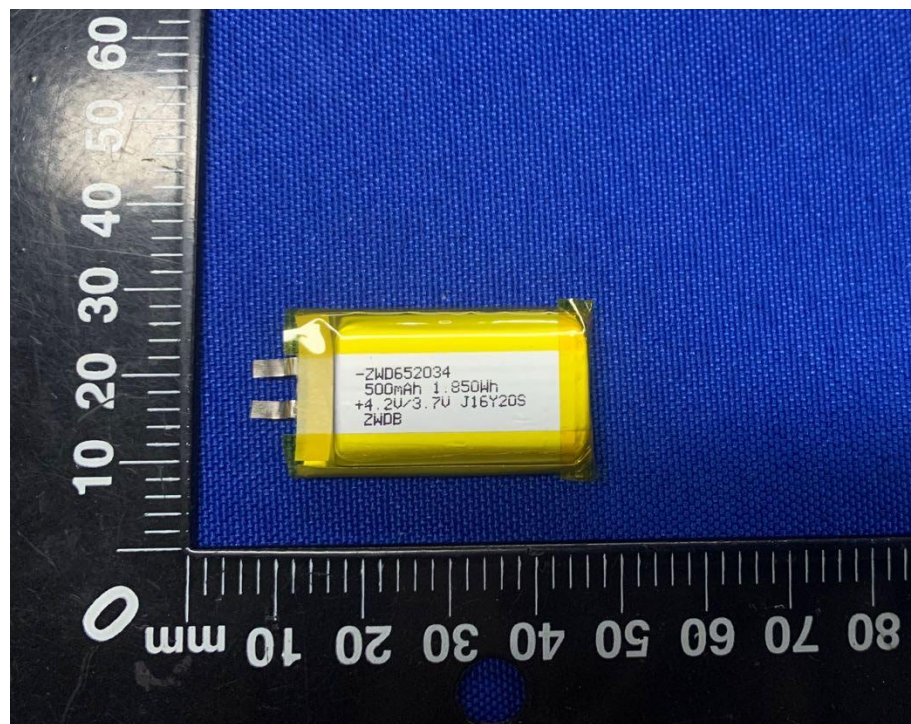
Picture 8 Front view of cell 图8: 电芯正面
