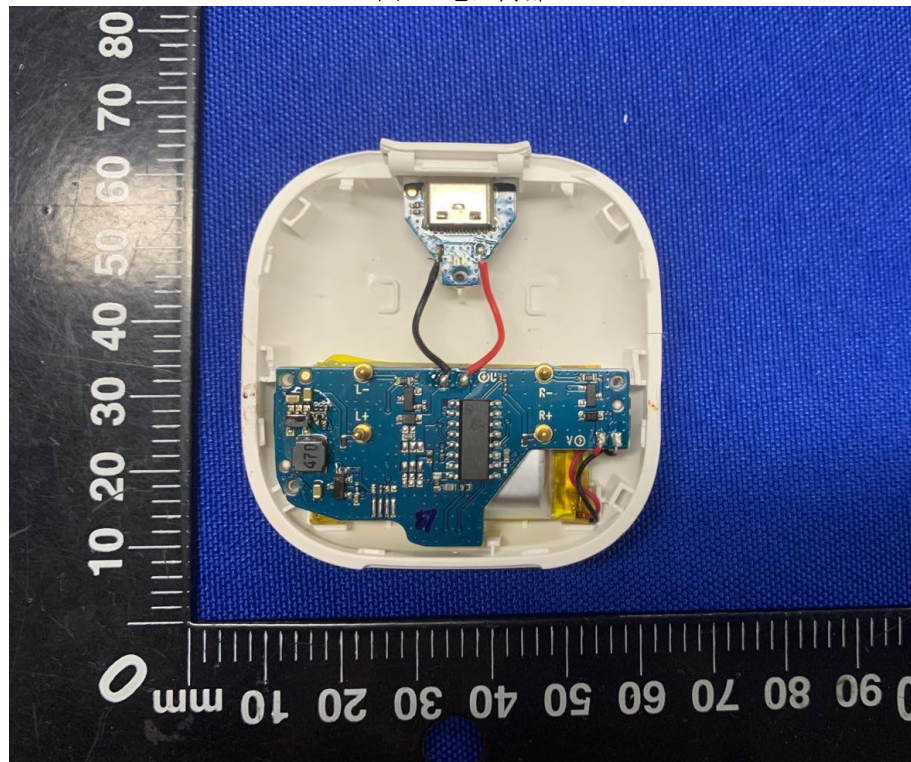
Picture 4 Inside view of battery
