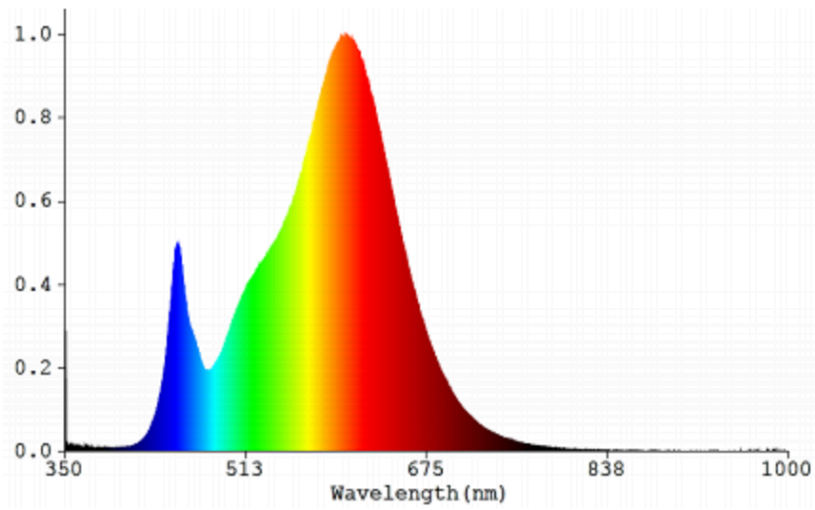
SMD2835-12C5B-0.5M-30
