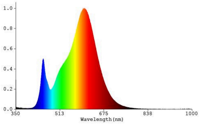
SMD2835-12C5B-0.5M-30
