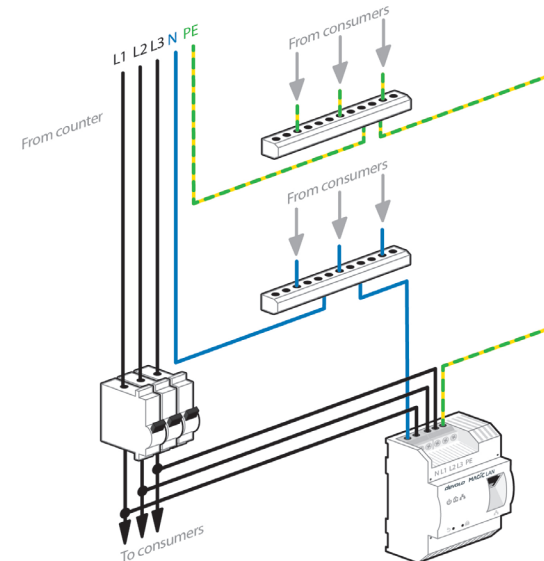
A) 3-phase installation without residual current circuit breaker
