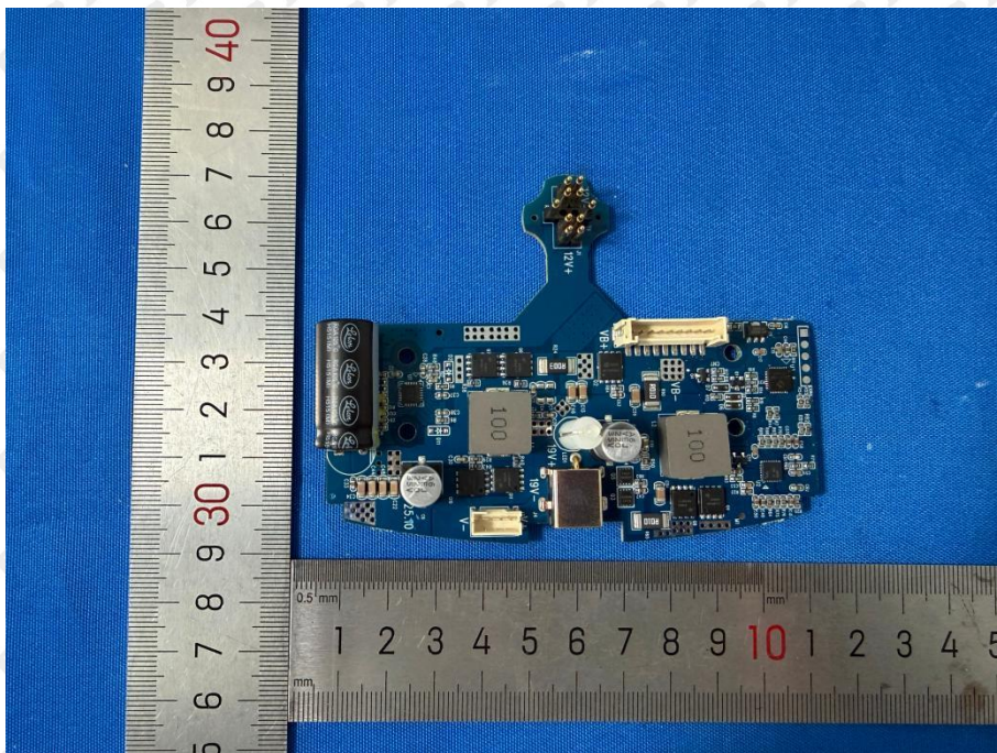
Photo 16: PCB view
