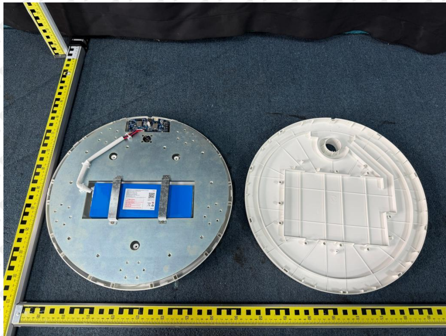
Photo 14: Internal view
