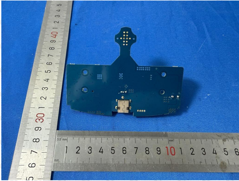
Photo 17: PCB view
