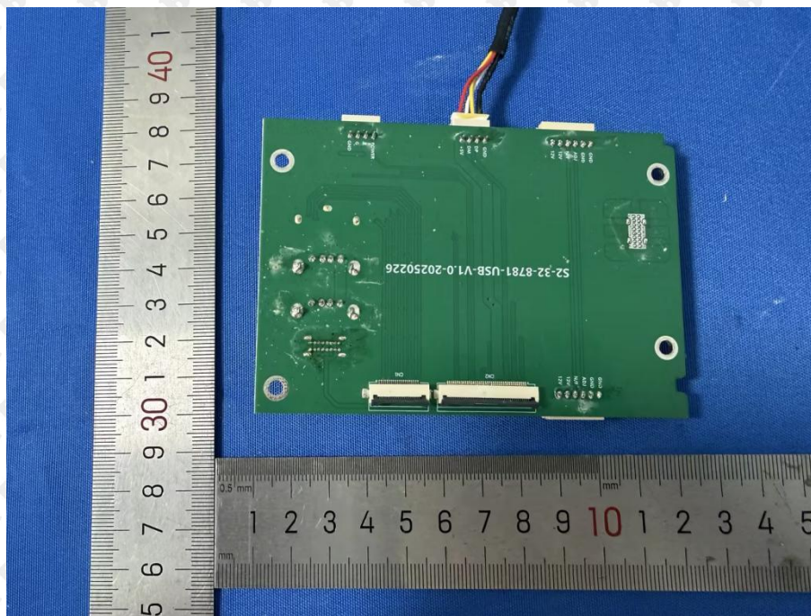
Photo 9: PCB view
