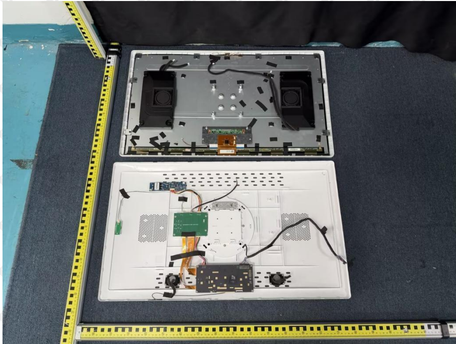
Photo 5: Internal view
