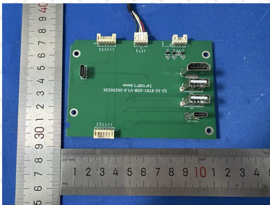
Photo 8: PCB view
