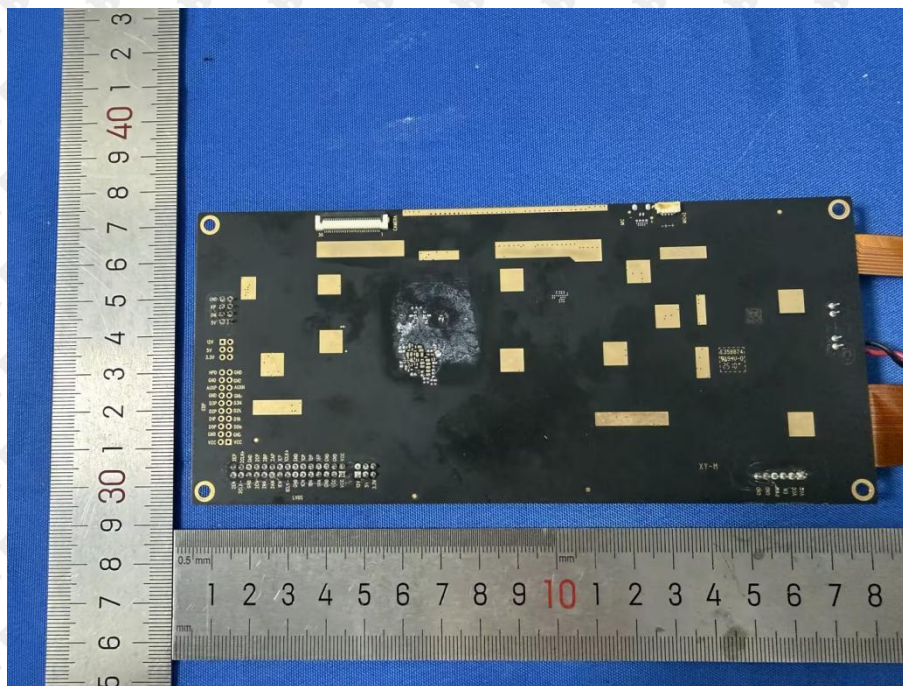
Photo 7: PCB view
