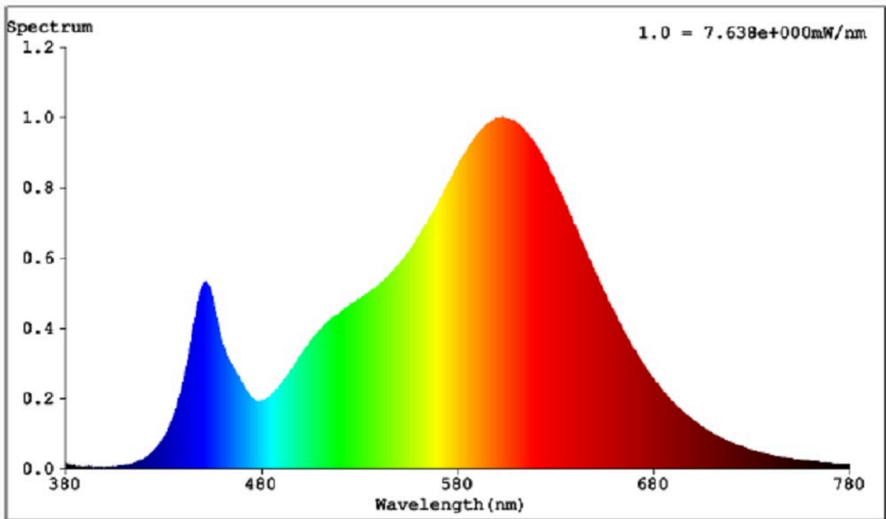
Spectral power distribution for light source of 9100C 5000K:
