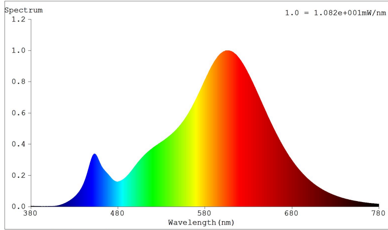
Spectral Distribution
