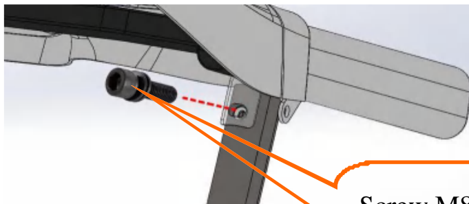
Screw M8*25
