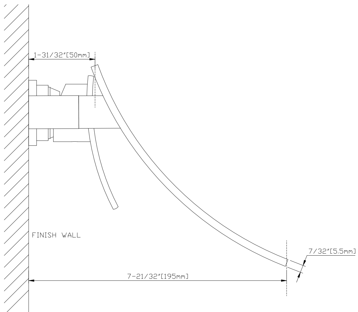
SIDE VIEW OF FAUCET
