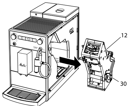
Fig. 16: Removing the brewing unit
