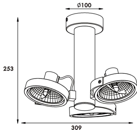
104806 3xG9 LED Max.3W
