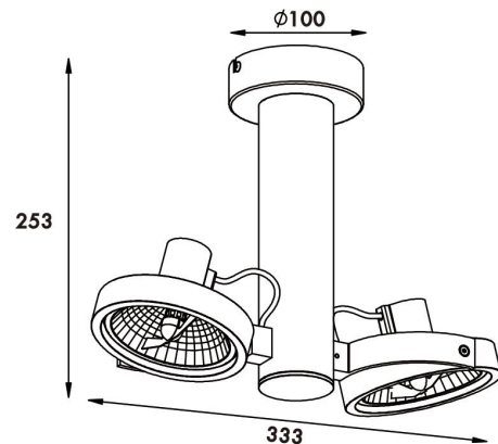
104805 2xG9 LED Max.3W
