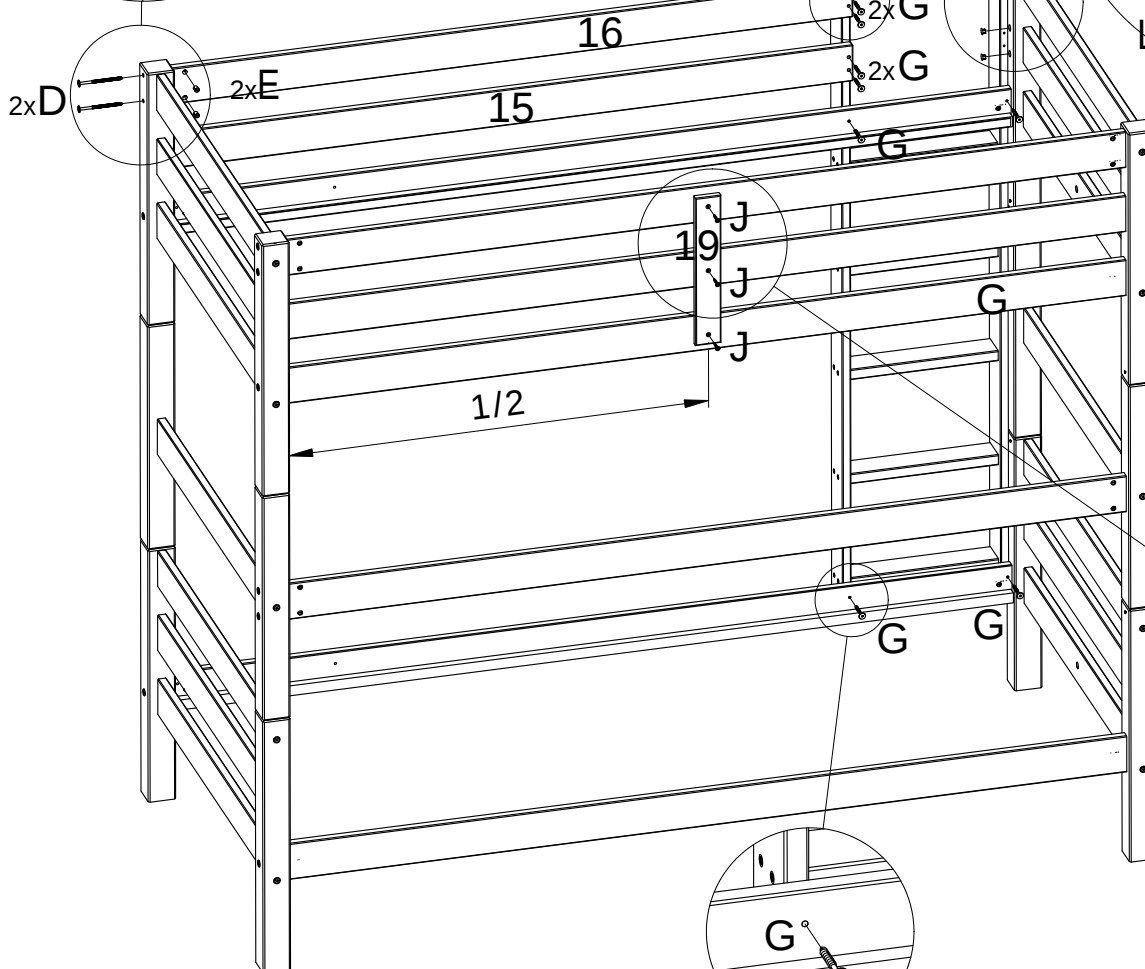
ASSEMBLING LADDER LEFT
