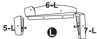
5 6 7 Arm Frame R&L * 6pcs
