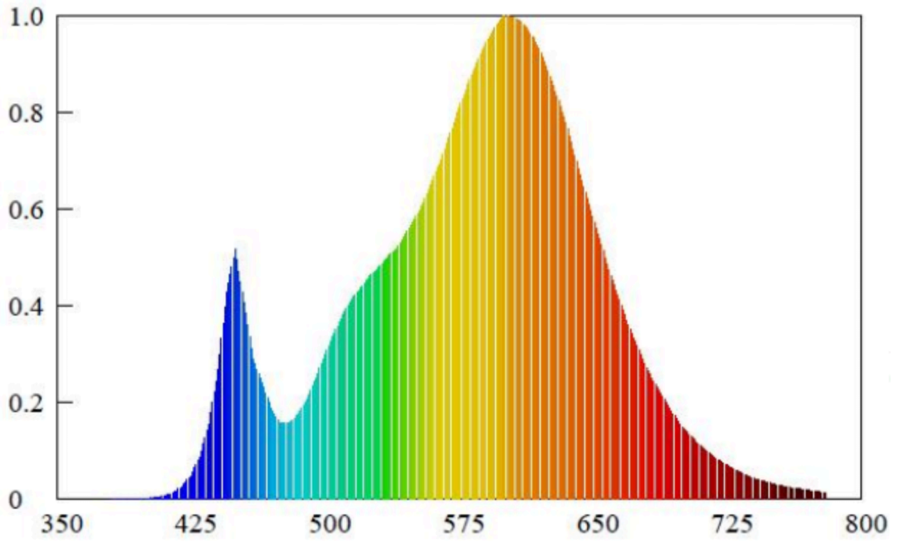
Spectral power distribution (3000K)
