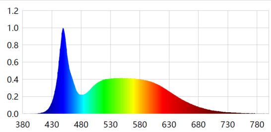
9507 CCT 3000K/6500K(6500K): 1#
