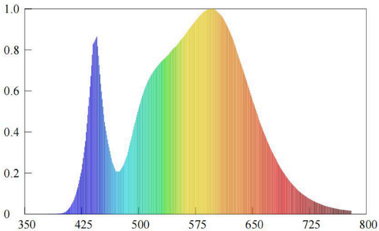
Spectral power distribution(4000K)
