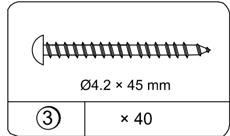
SCREW TCS1003
