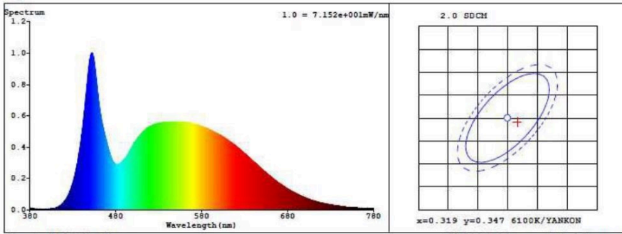
Spectral Distribution
