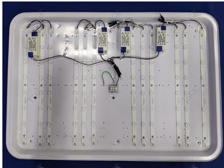
Internal structure for model 30814401-1
