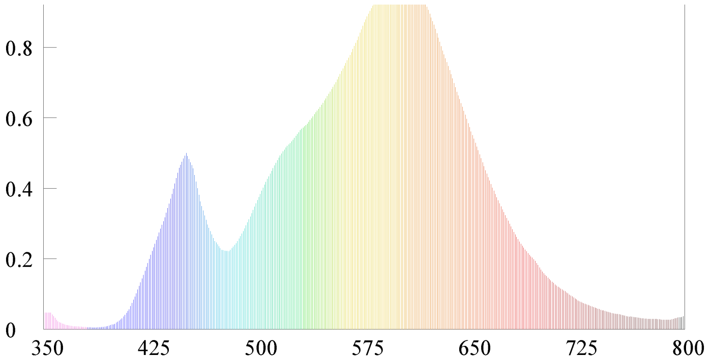
Spectral Distribution
