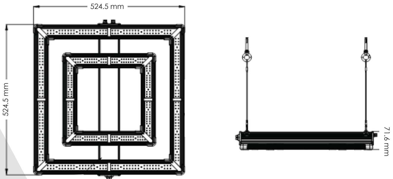
Fig 1. Fixture dimensions
