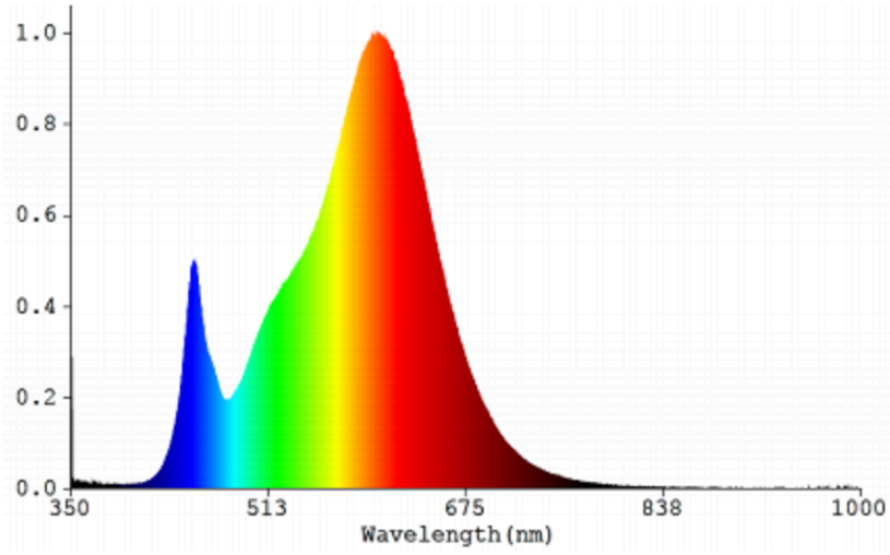
SMD2835-12C5B-0.5M-30
