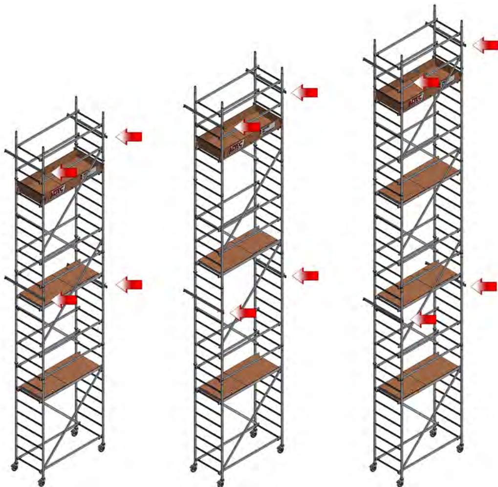
Rollfix 2.0 – 800/800 S
