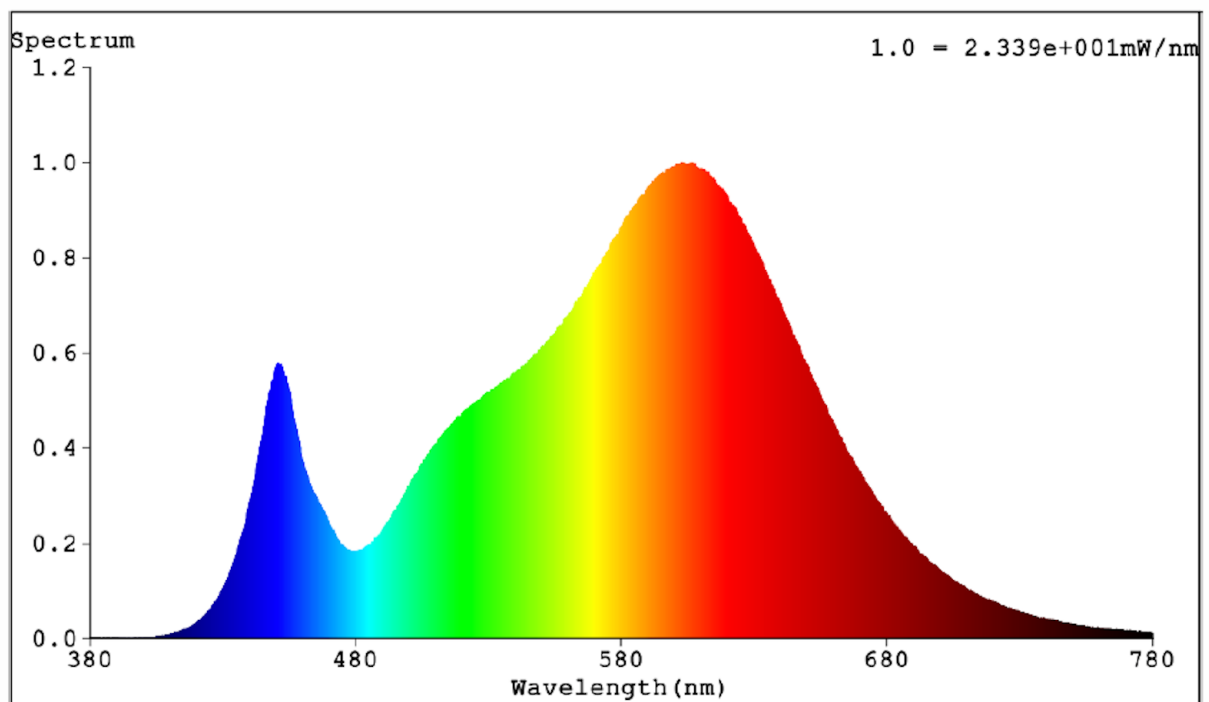
Data 3: Spectral power distribution for light source of MP-595X12-2835-9C6B:
