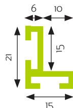
in Aluminium
