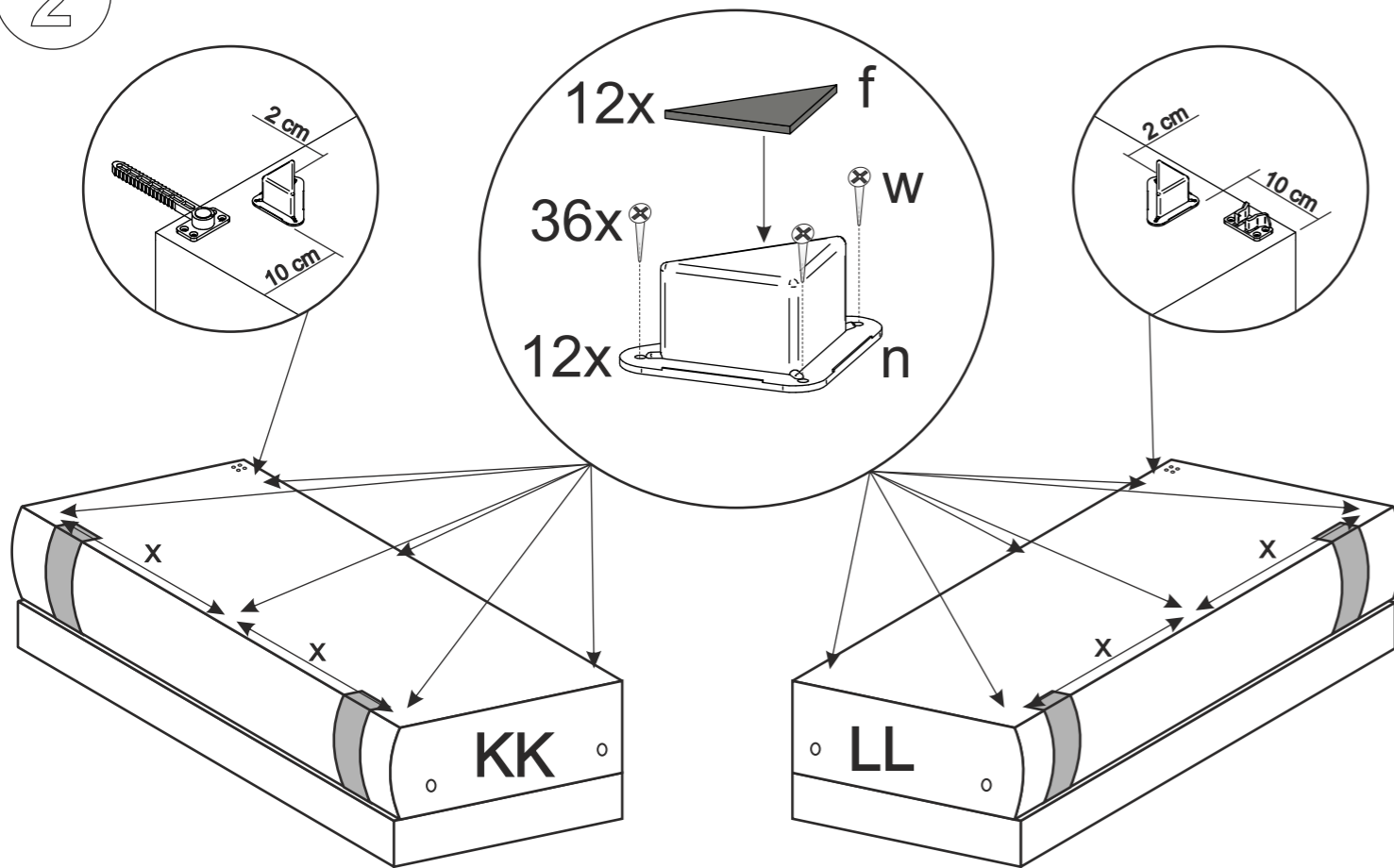
COPENHAGEN 180 LED
