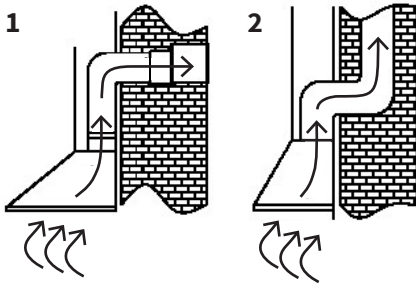
Fig. 1: Exhaust air to the outside
