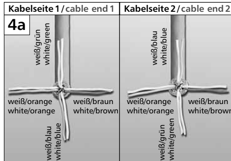
Je nach Austritt des Kabelendes Adernpaare separieren ... Separate the wire pairs on each end according to their exit from the sheath ...
