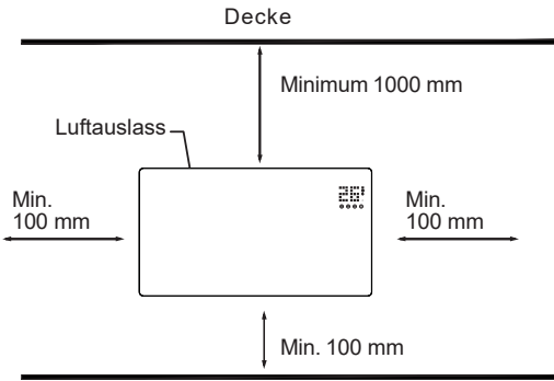
Wandmontage
