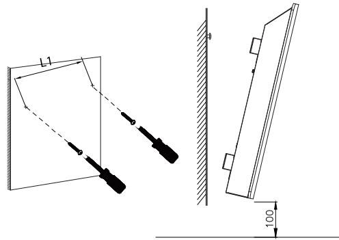
Wandmontage
