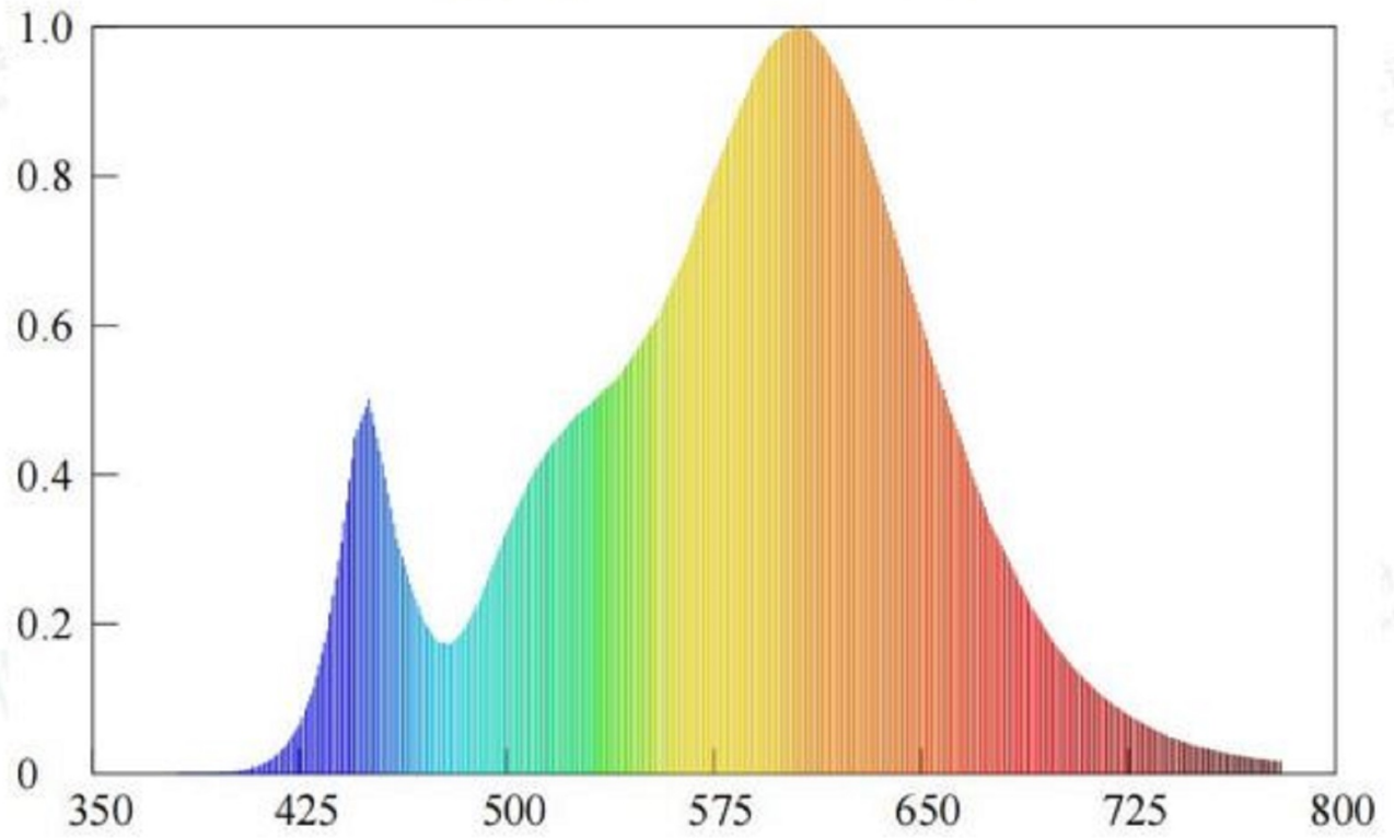
Spectral power distribution(3000K)
