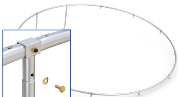
fig. 4: Screw feet to frame
