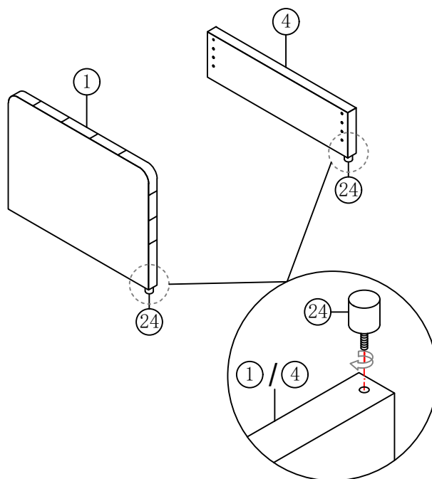
Head board on the left Kopfplatte links Plaque de tête gauche
